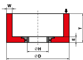
6001 - D × T × H - W...E...
