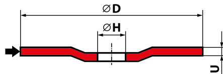
42 - D x U x H
