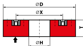
36 - D × T × H
