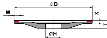
12A2PA - D × T-X × W × X × H
