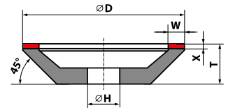
12A2-45 - D × T-X × W × X × H
