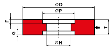
7 - D \times T \times H - P...F...G...
